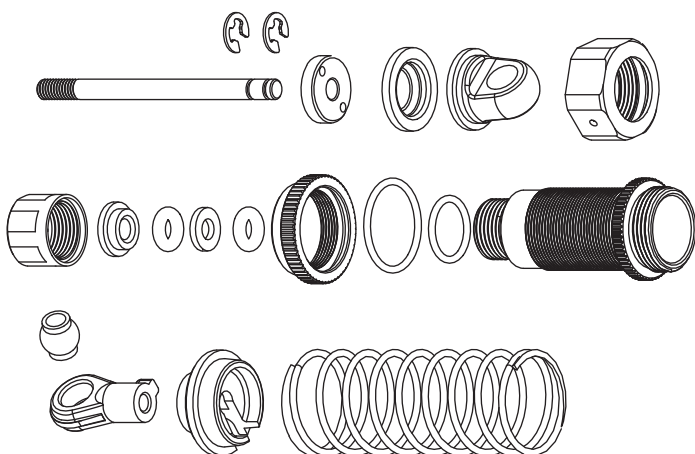
Front Shock Absorber (前避震器) 2PCS
