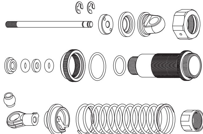
Rear Shock Absorber (後避震器) 2PCS
