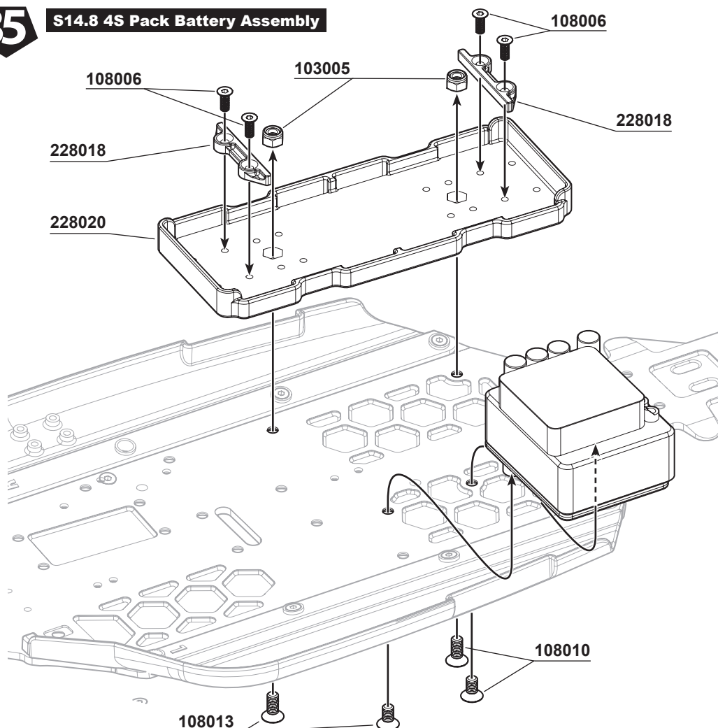
108010 M4x10mm FH/ST HEX Screw x2
