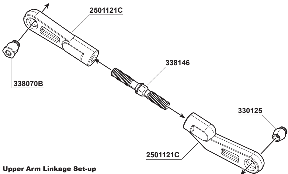
338146 Rear Upper Sus. Arm Turnbuckles x2
