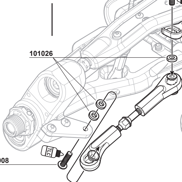
106008 M3x12mm Hex Scket OH/TP Screw x2
