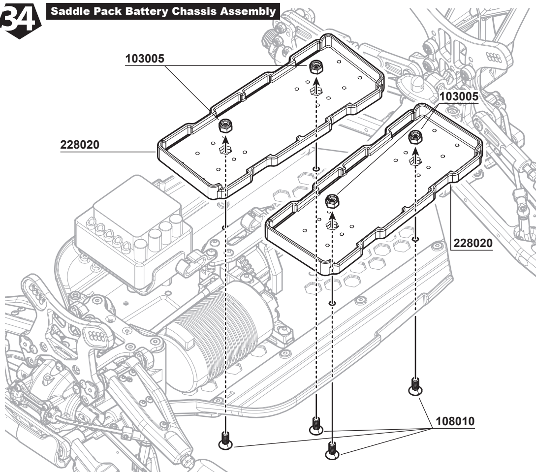
108010 M4x10mm FH/ST HEX Screw x4
