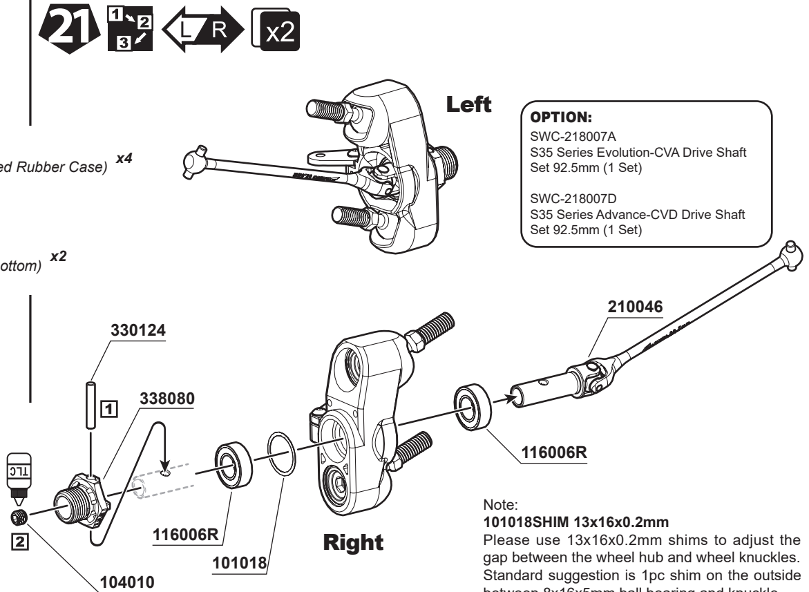
101018 SHIM 13x16x0.2mm x2
