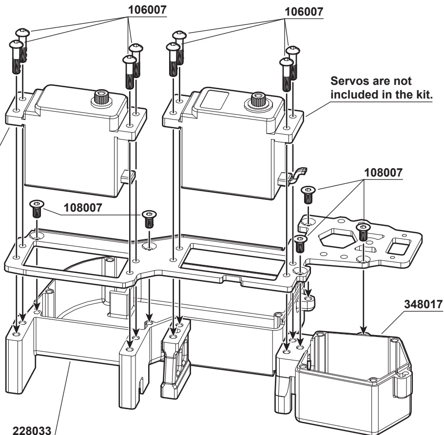
106007 M3x12mm Hex Socket OH/TP Screw(HT) x8
