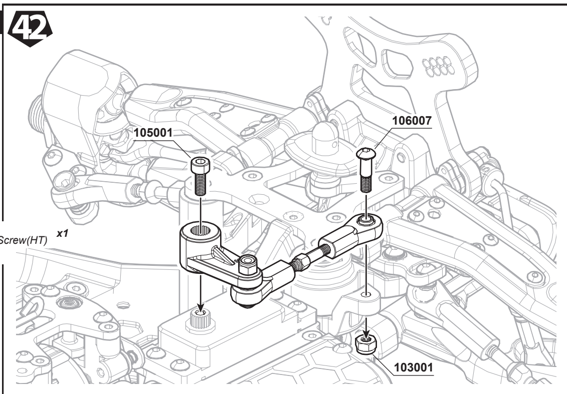
105001 M3x10mm Cap Screw x1
