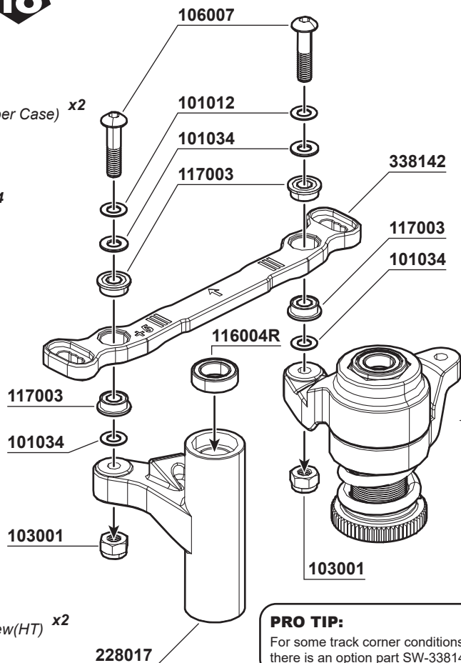
117003 Flange Ball Bearing 3x6x2.5mm x4
