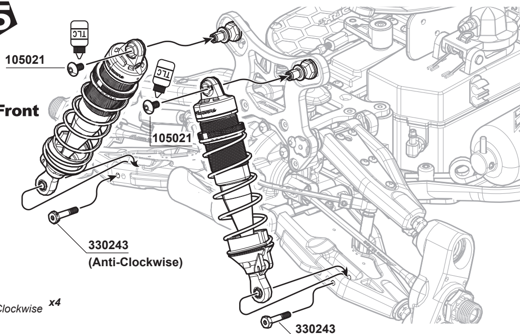
105021 M3x6mm Conical Head Screw x4
