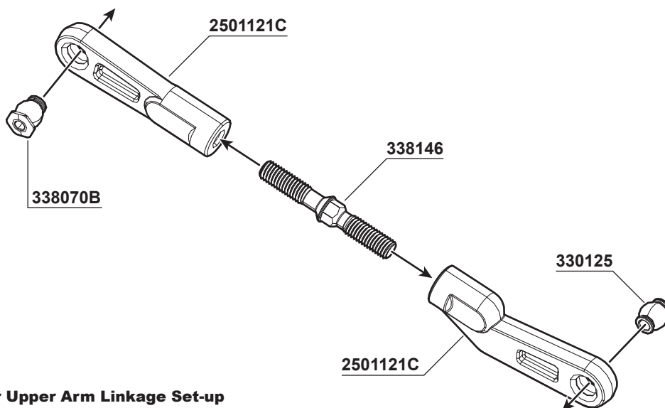
338146 Rear Upper Sus. Arm Turnbuckles x2
