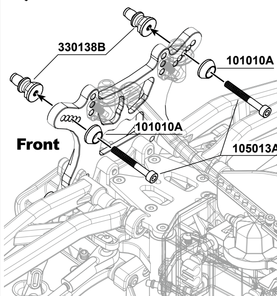
105013A M3x25mm Cap Screw x4
