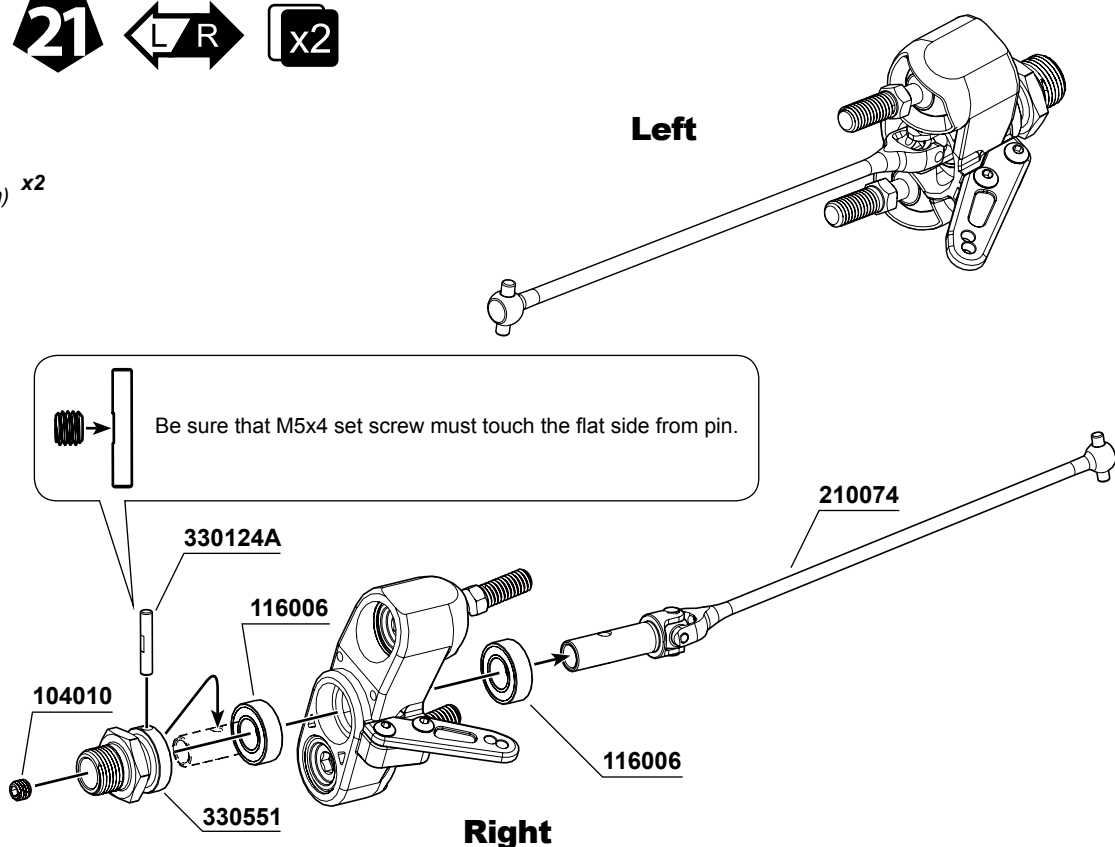
116006 Ball Bearing 8x16x5mm x4
