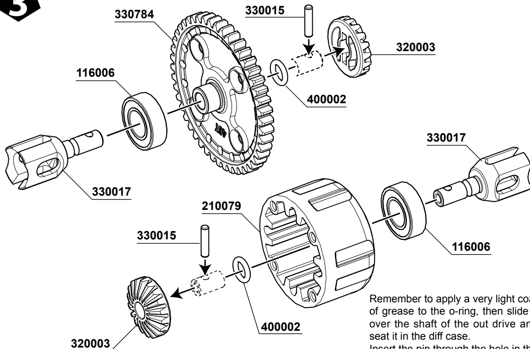
116006 Ball Bearing 8x16x5mm x2
