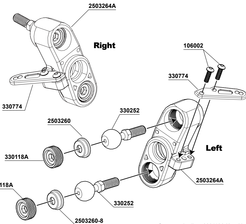
106002 M3x10mm Hex Socket OH/TP Screw x4
