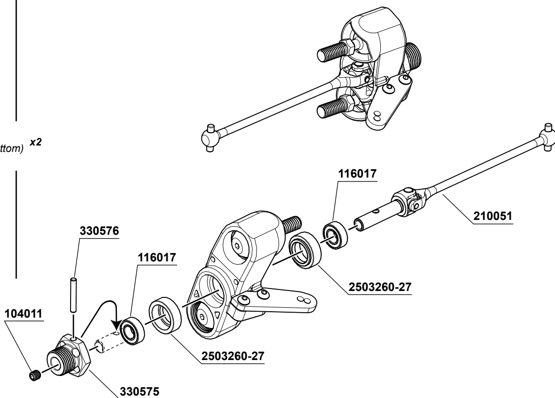
116017 Ball Bearing 6x12x4mm x4
