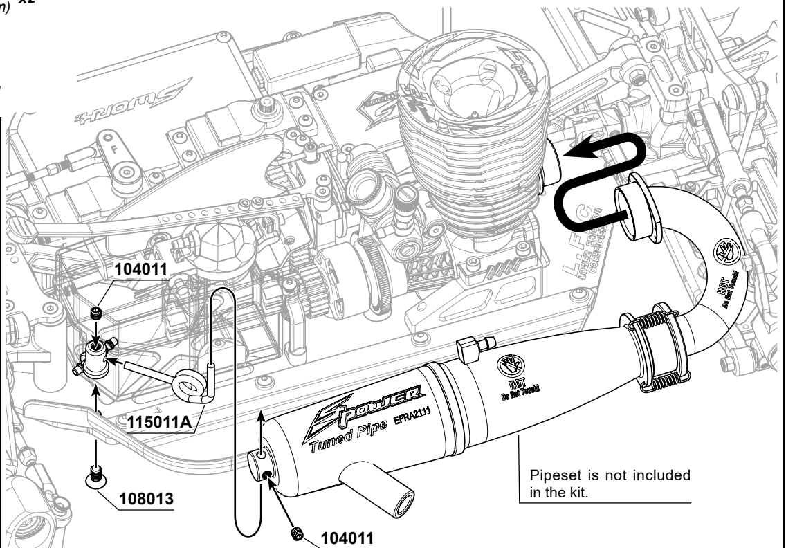
108013 M4x8mm FH/ST HEX Screw x1
