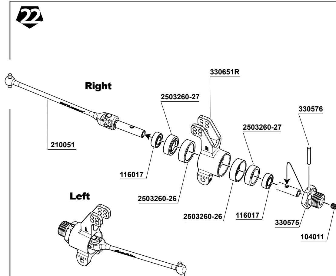
116017 Ball Bearing 6x12x4mm x4
