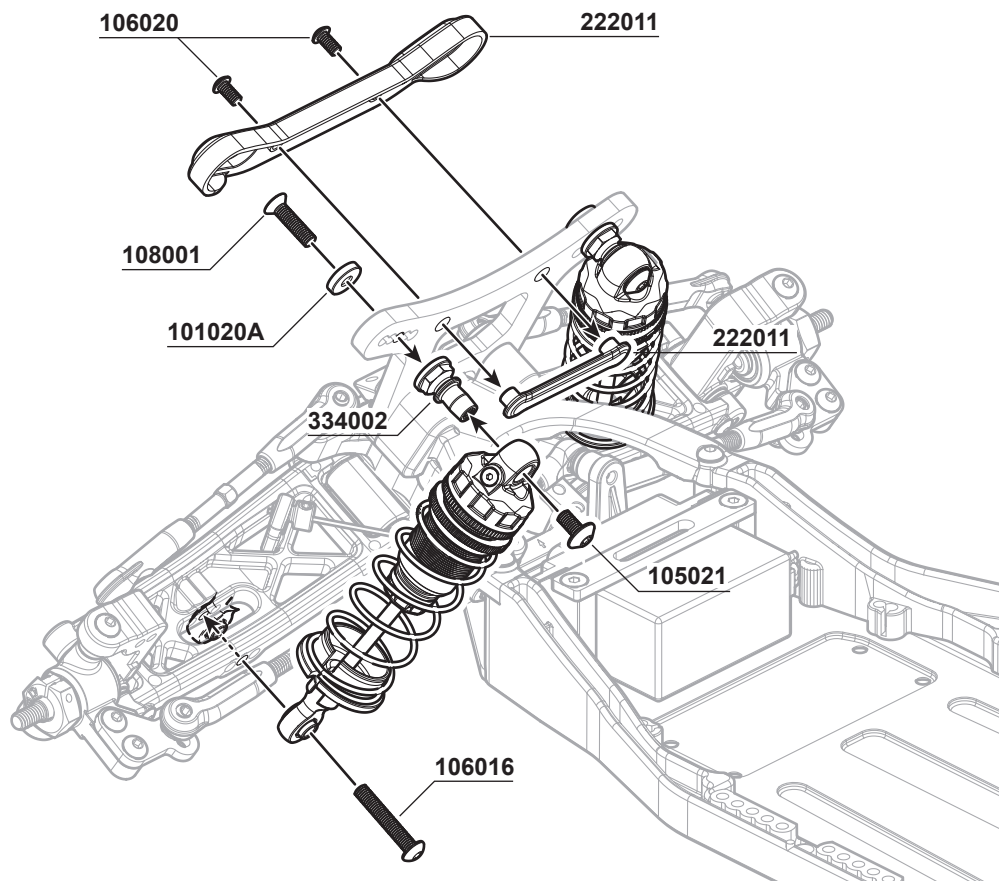
106020 M2.5x5mm Hex Socket OH/TP Screw x2
