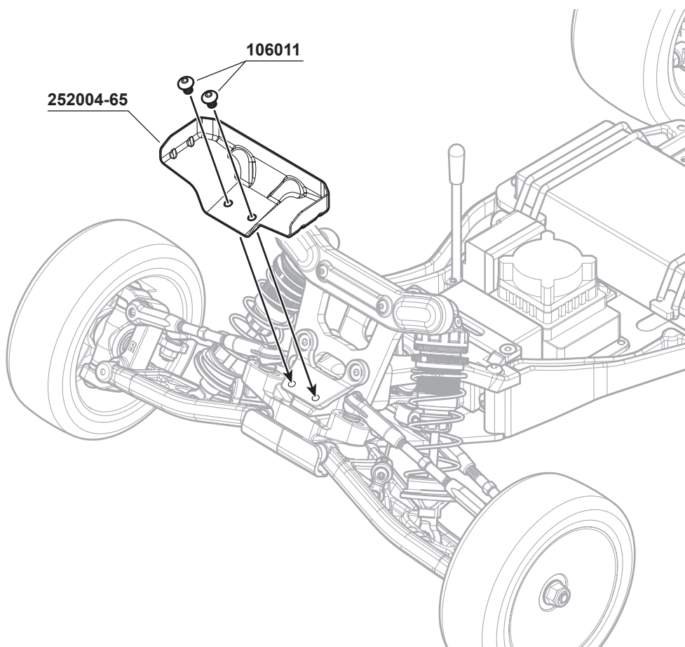
106011 M3x4mm Hex Scket OH/ST Screw x2
