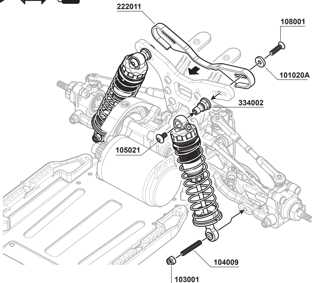
101020A 3mm Countersunk Washers (GM) x2
