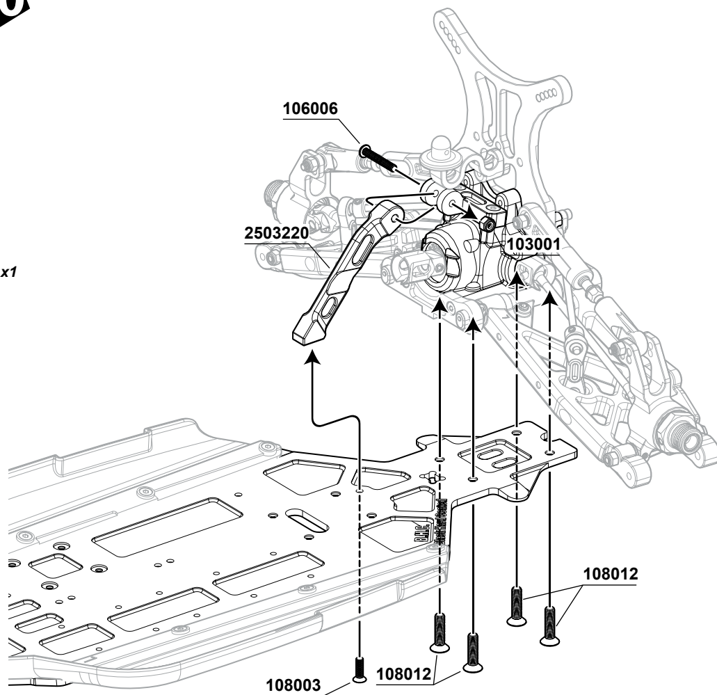
108012 M4x16mm FH/ST HEX Screw x4
