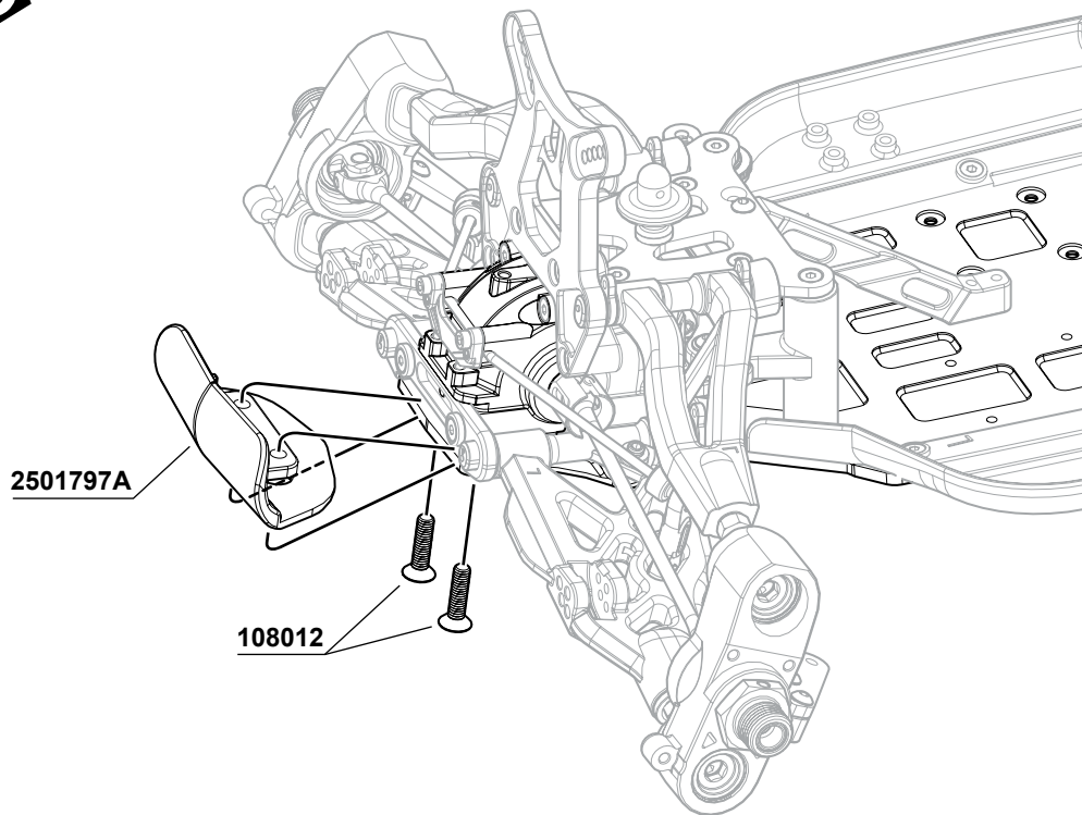
108012 M4x16mm FH/ST HEX Screw x2
