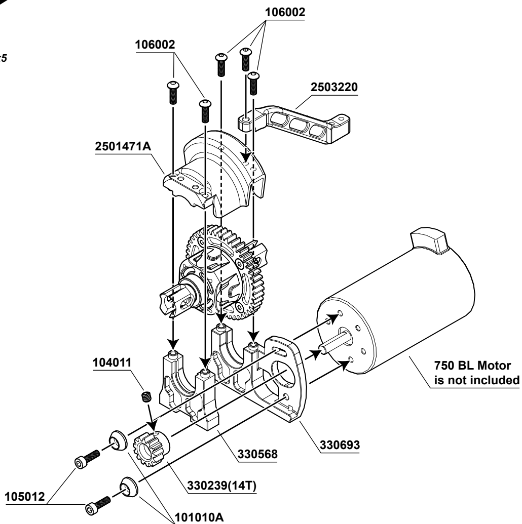
104011 M4x4mm Set Screw (Flat Bottom) x1
