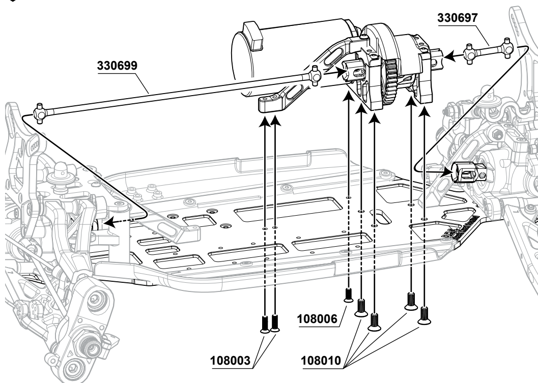
108010 M4x10mm FH/ST HEX Screw x4
