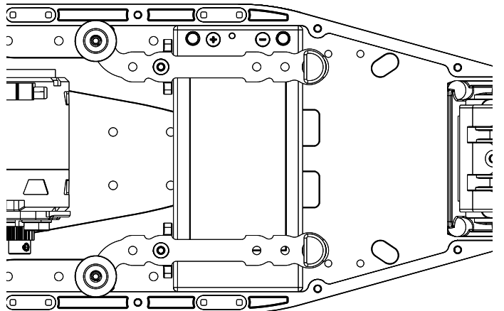
36.9mm Battery Shift. Forward Posts - Forward Lipo
