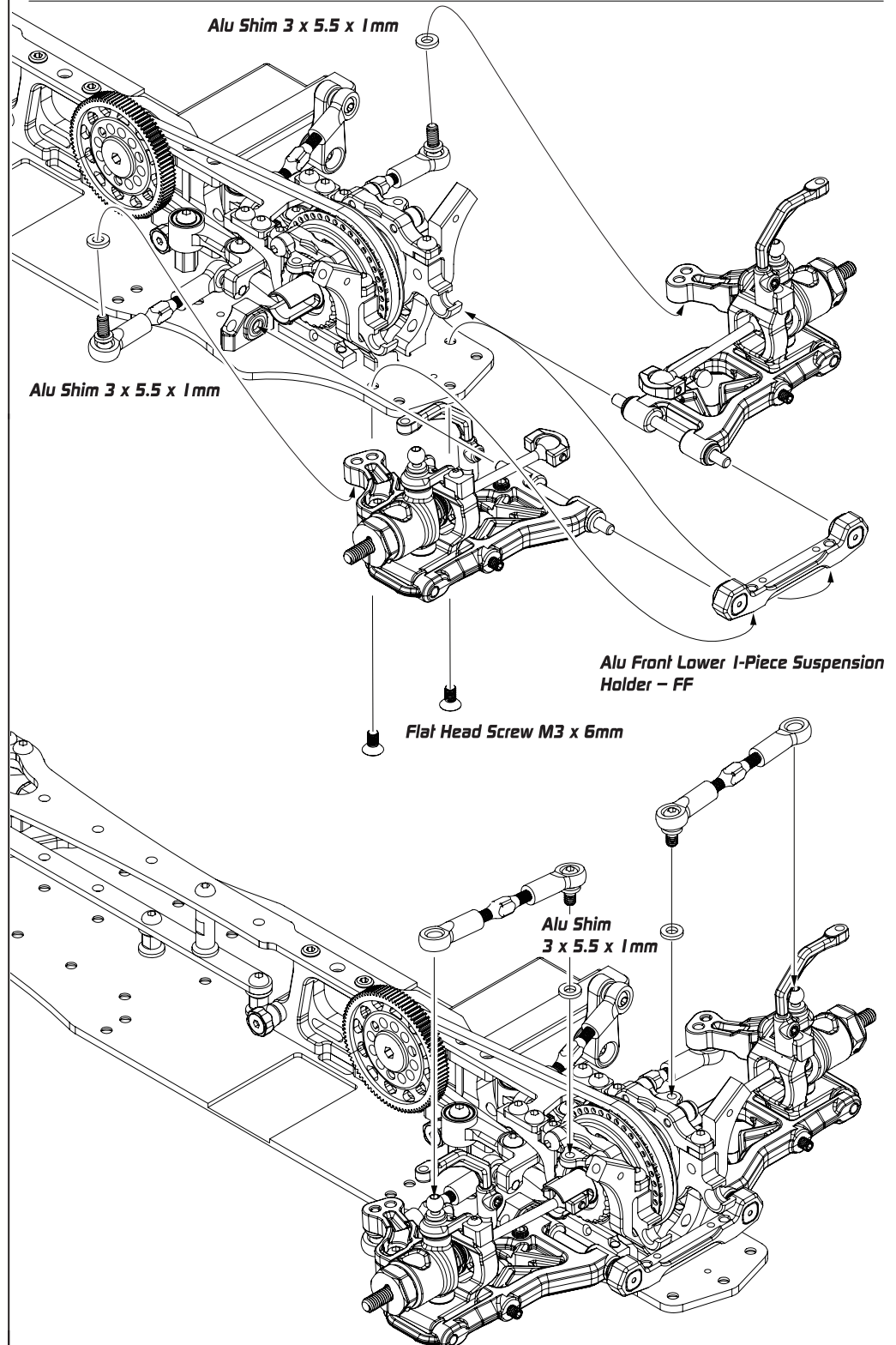
Alu Front Lower I-Piece Suspension Holder – FF
