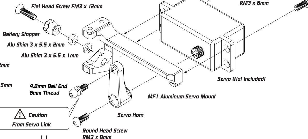
Aluminum Shim 3x5.5x1.0mm XP-10240
