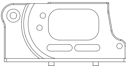
MF1 Aluminum Motor Mount XP-10964
