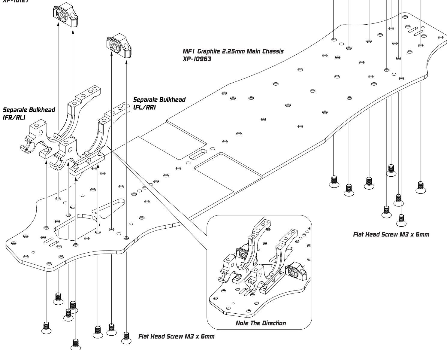
Eccentric Bushing Set XP-10127
