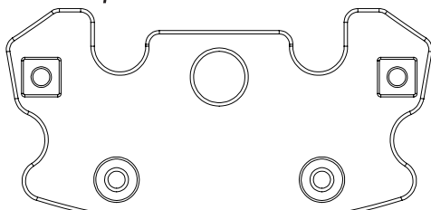
Brass Lower Bumper Plate ( 90g ) XP-10927
