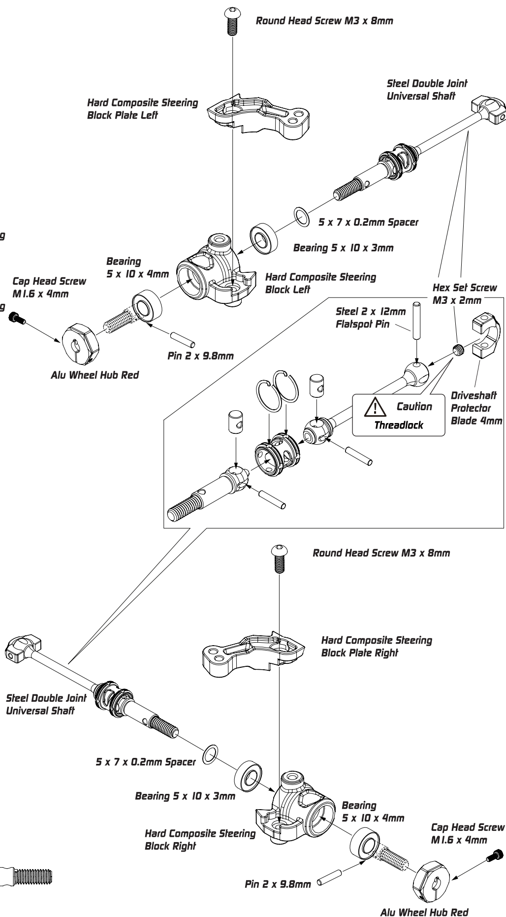
Hard Composite Steering Block Left XP-10247
