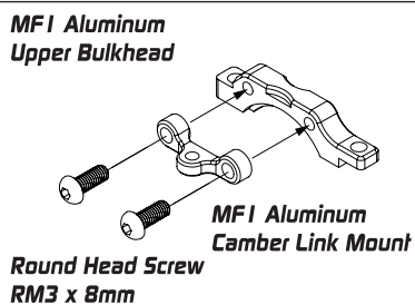
Round Head Screw RM3 x 8mm
