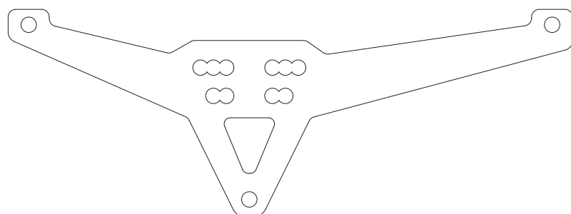
Lightning10X235 Upper Pod Plate A-01-P51720 x 1
