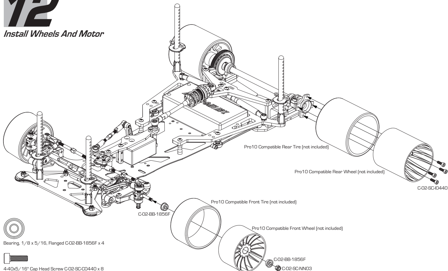
4-40x5/16" Cap Head Screw C-02-SC-C0440 x 8
