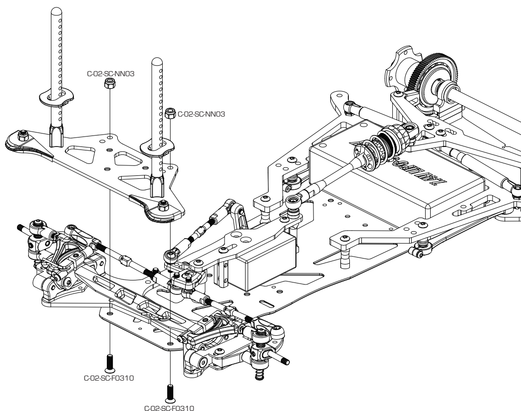
M3x10mm Flat Head Screw C-02-SC-F0310 x 2
