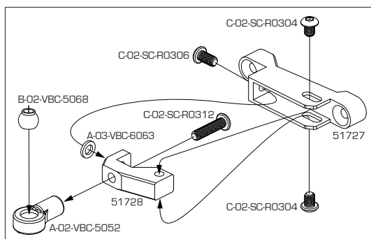
Lightning WGT ALU7075 Steering Knuckle B-02-P50233 x 2
