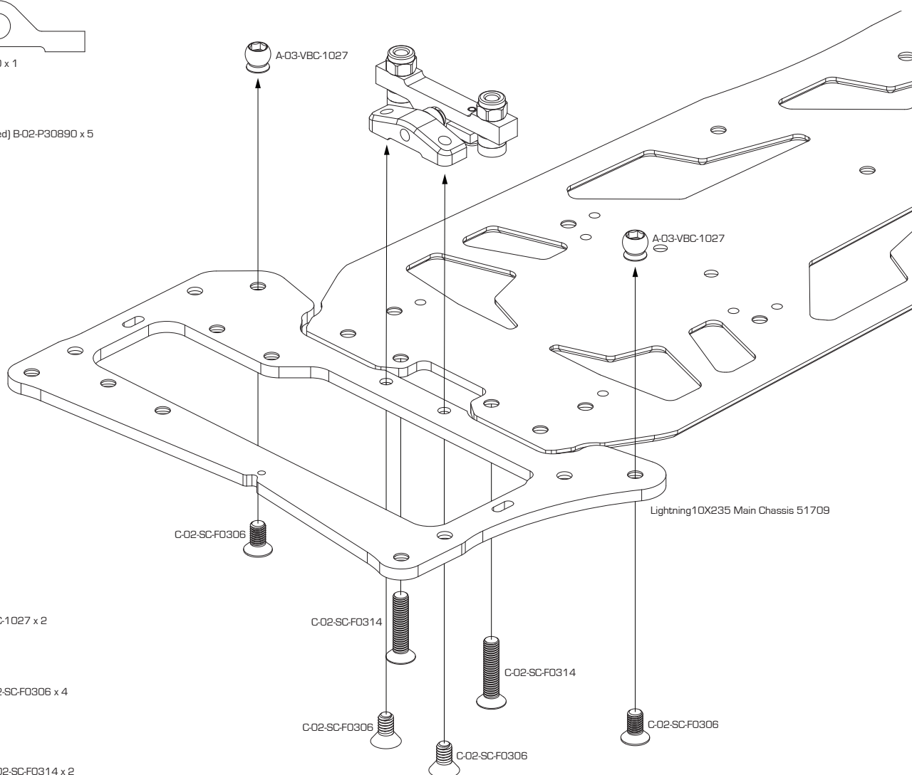
M3x14 Flathead C-02-SC-F0314 x 2
