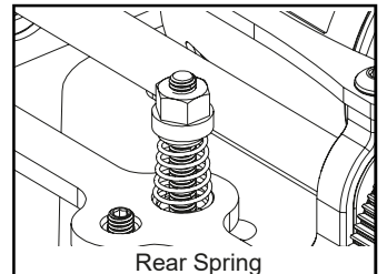
Rear Spring
