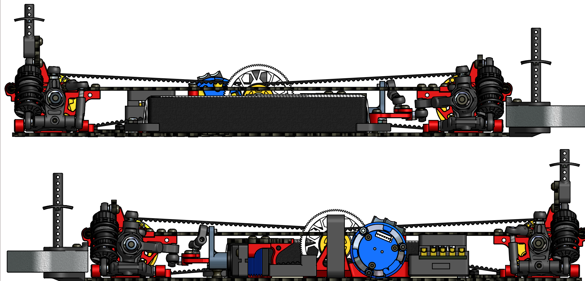
- Final Assembly View - Capricorn RC
