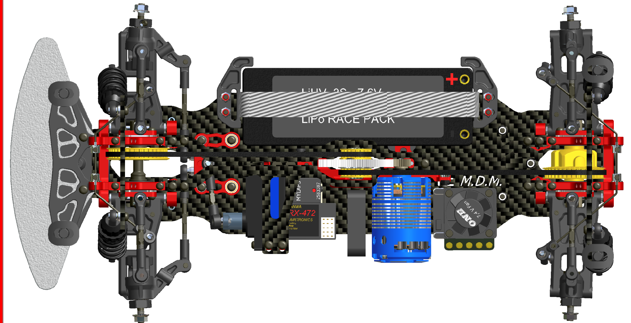
- Final Assembly View - Capricorn RC
