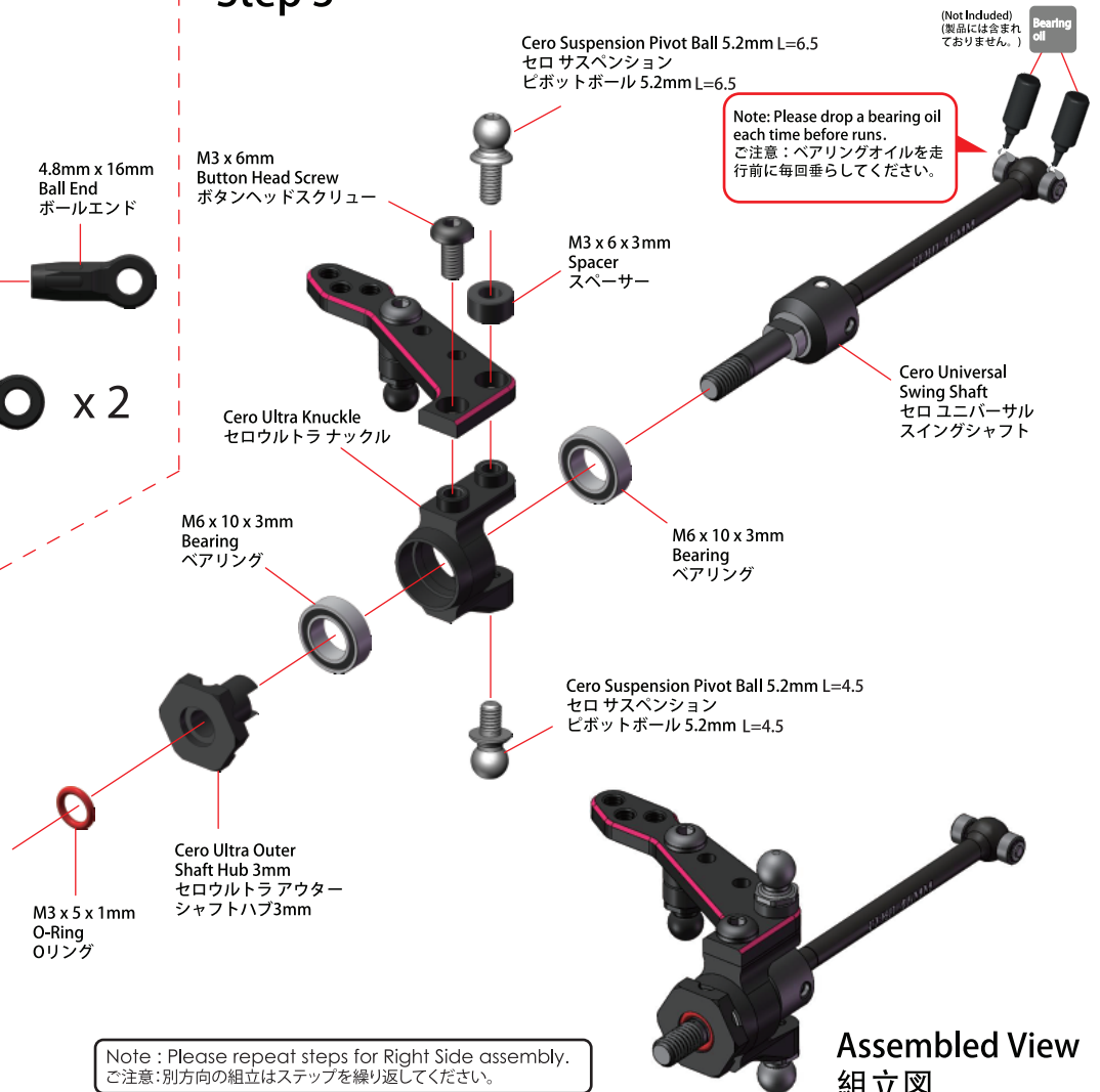
Assembled View 組立図
