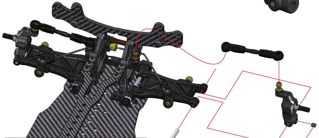
Assembled View 組立図
