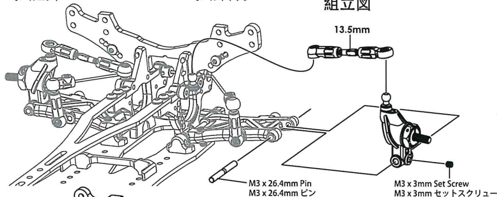
Assembled View 組立図
