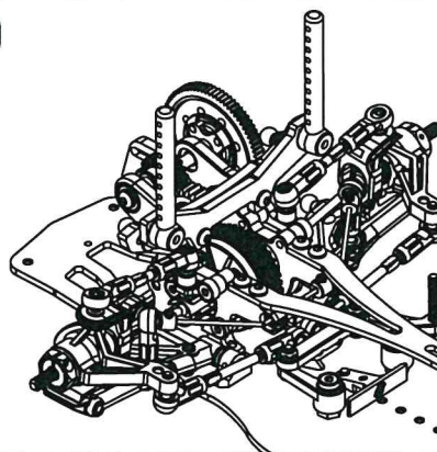
Assembled View 組立図
