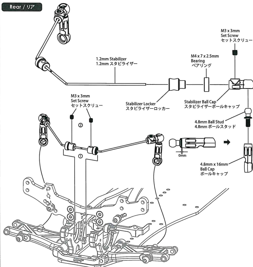
Assembled View 組立図
