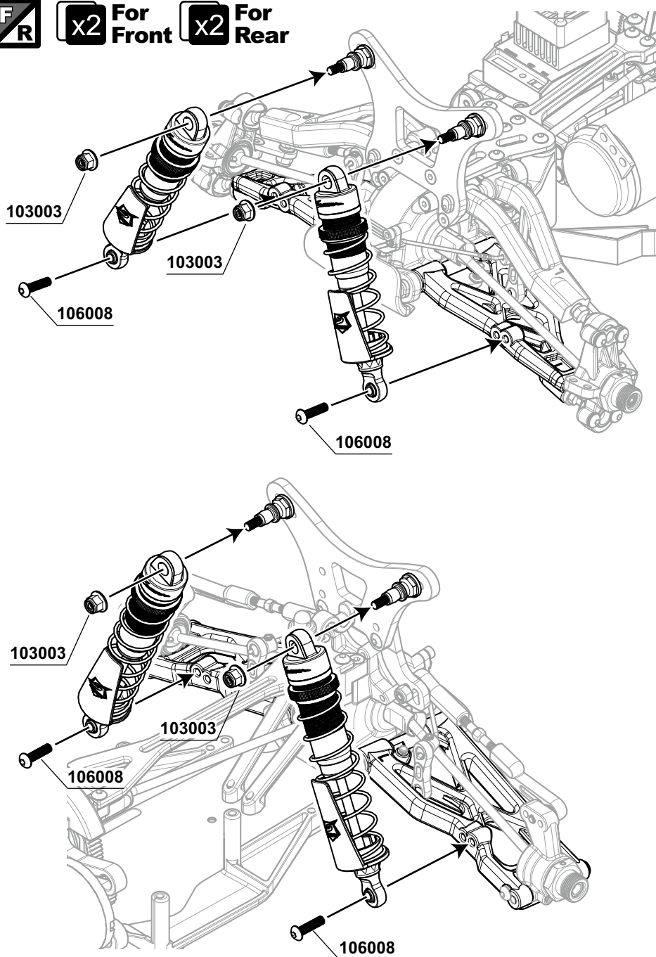
106008 M3x12mm Hex Scket OH/TP Screw x4
