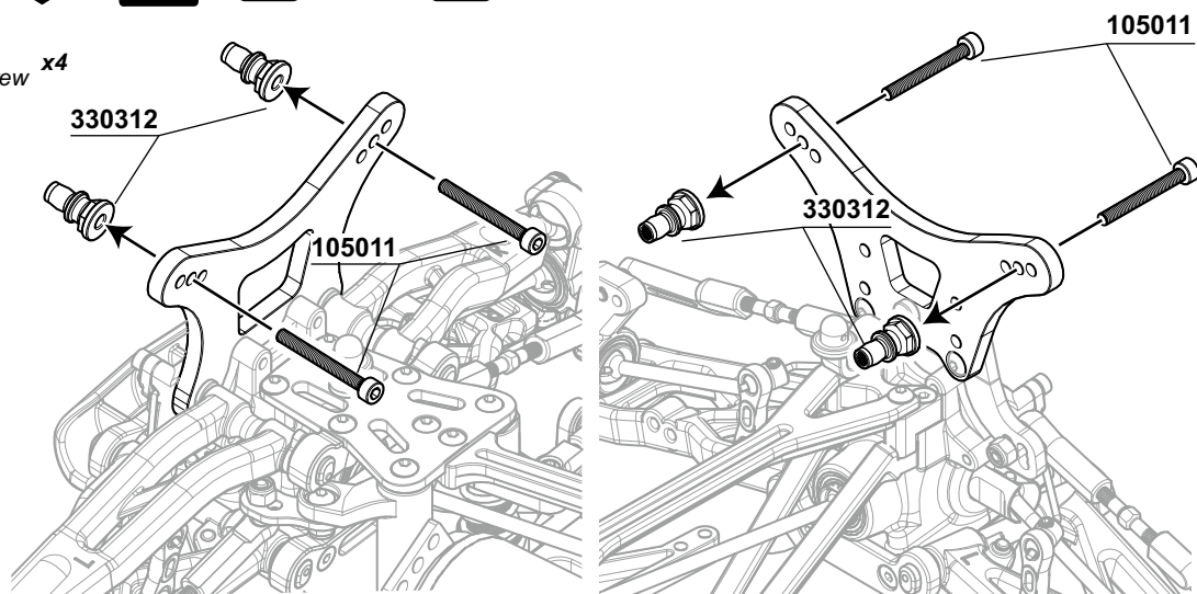
330312 Aluminum Shock Cap Studk x4
