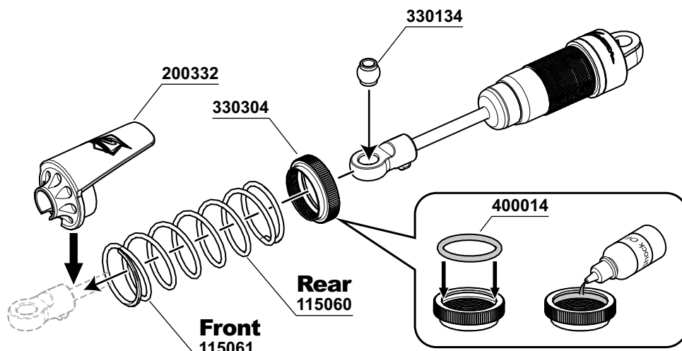
330304 Aluminum Shock Spring Adjust Nut x4
