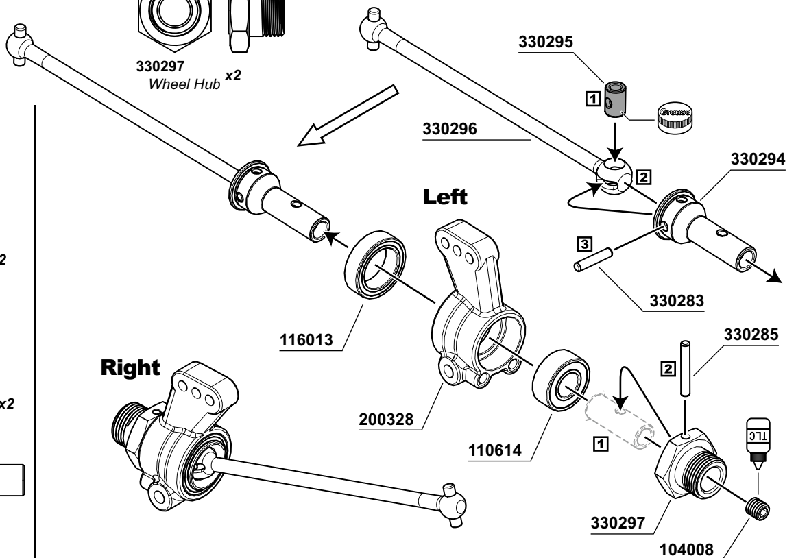
330296 F/R Drive Shaft 78mm x2
