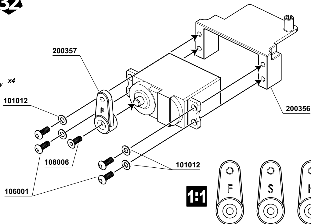
108006 M3x8mm FH/ST HEX Screw x1
