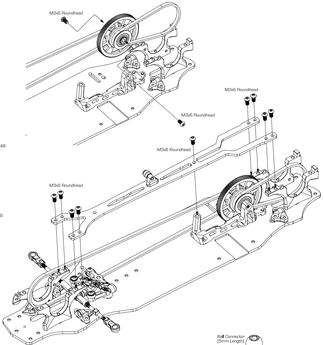
WildFireD07 Rear Upper Bulkhead, Left B-02-P30149
