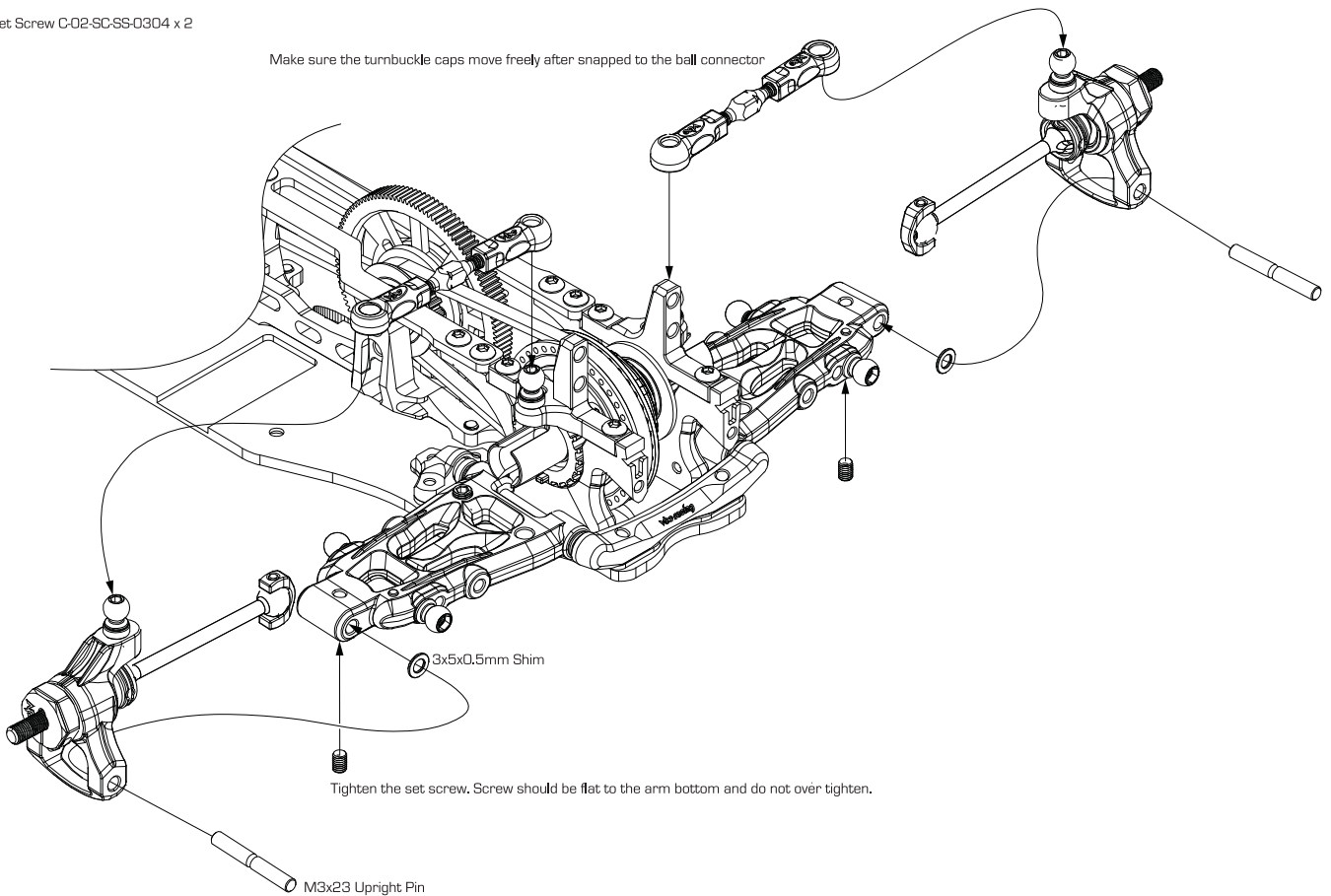
M3x23 Upright Pin
