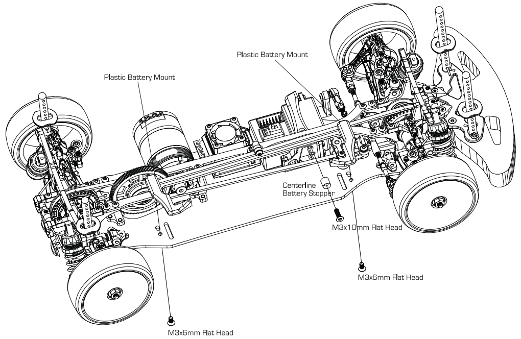
Centerline Battery Stopper B-02-VBC-3034 x 1
