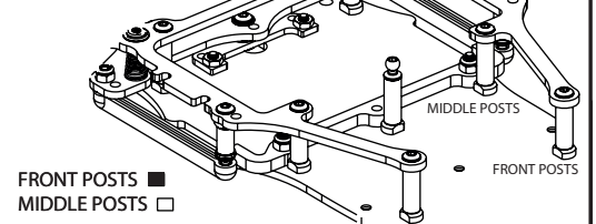
TOPDECK STIFFNESS ADJUSTMENT
